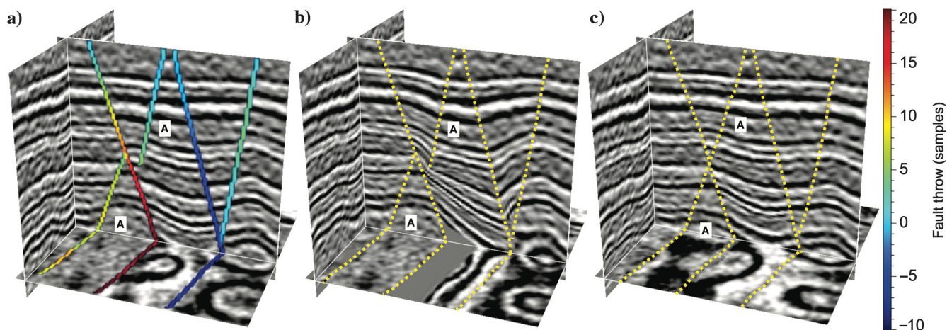
Figure 1. (a) A 3D synthetic seismic image with faults colored by fault throws is significantly distorted when (b) unfaulted by moving only fault blocks while fixing fault positions. (c) Faults (especially fault A) must also be moved to obtain an unfaulted image with minimal distortions.
