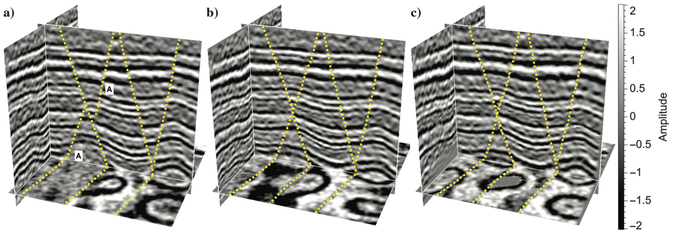
Figure 8. (a) The input synthetic seismic image is (b) unfaulted using shifts in Figure 6 computed by method 1, and (c) using shifts in Figure 7 computed by method 2.
