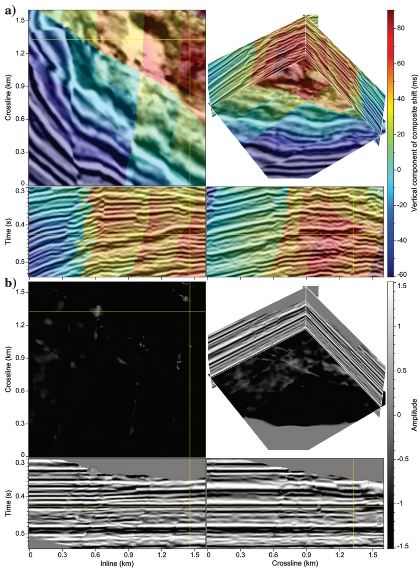
Figure 11. (a) Composite shifts are computed and then used to obtain (b) an unfaulted and unfolded image.
