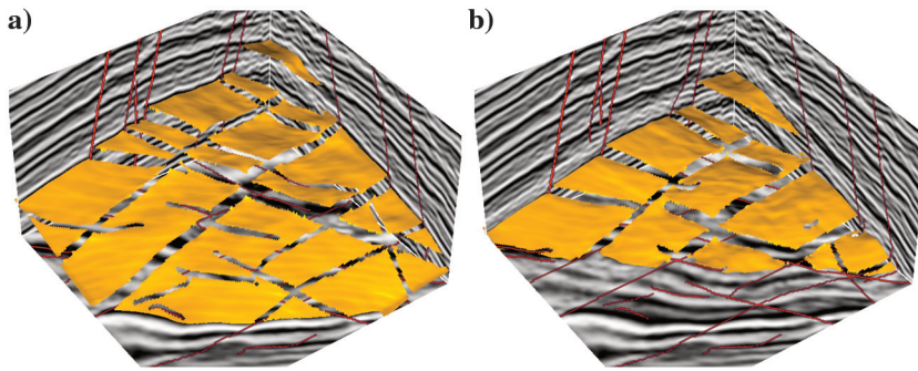
Figure 12. Two horizon surfaces (colored by yellow depth) are extracted using composite shift vectors that map an image from input space to unfaulted and unfolded space. The vertical component of the composite shift vectors is displayed in Figure 11a.
