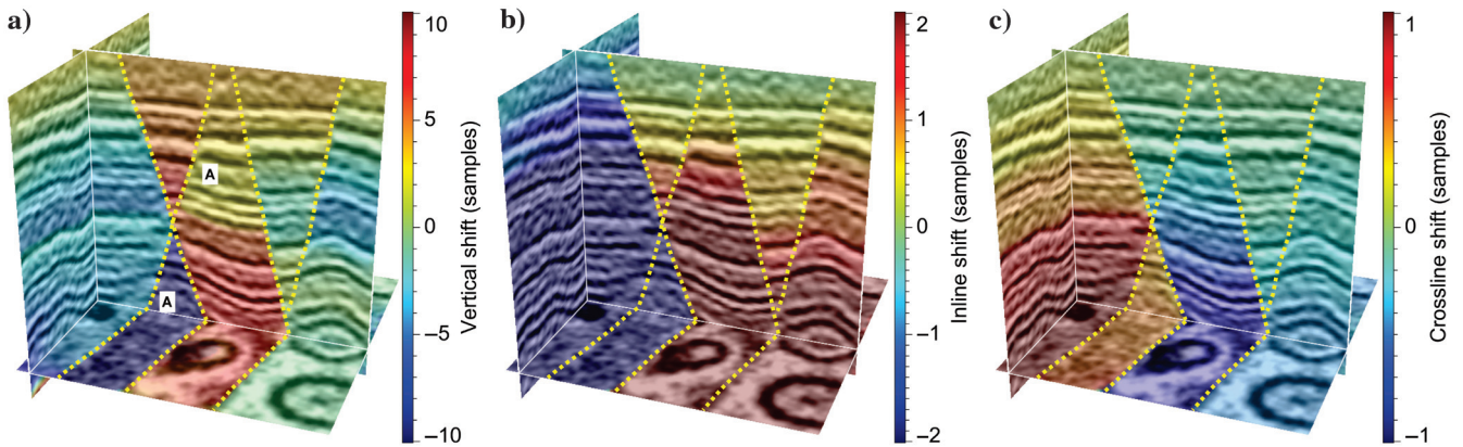
Figure 7. (a) Vertical, (b) inline, and (c) crossline components of unfauling shifts in the unfaulted space are converted from those in the input space shown in Figure 5. The discontinuities on each component of shifts are displaced relative to those in Figure 5.
