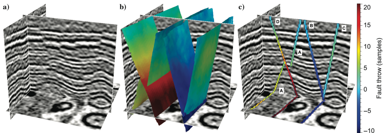
Figure 2. (a) Given a 3D seismic image, we extract (b) fault surfaces and estimate fault dip slip vectors for each sample on fault surfaces. Faults in panels (b) and (c) are colored by fault throws, the vertical components of slip vectors.
