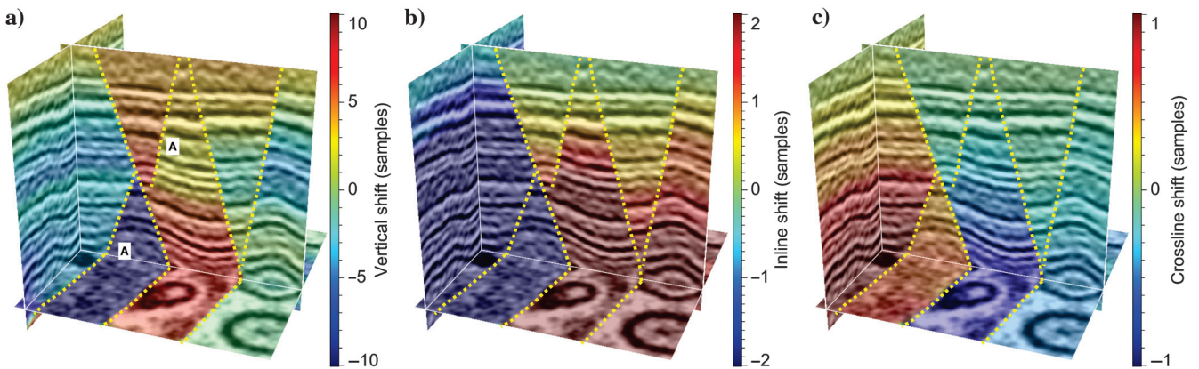
Figure 5. (a) Vertical, (b) inline, and (c) crossline components of unfauling shifts \mathbf{s}(\mathbf{x}) are computed in the input space using method 2. Discontinuities in each component of shifts coincide with fault locations.
