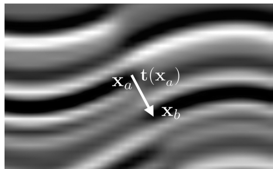
Figure 3. A fault slip vector \mathbf{t}(\mathbf{x}_a) , estimated at each footwall sample adjacent to a fault, tells us how to correlate the image sample at \mathbf{x}_a in the footwall to the corresponding sample \mathbf{x}_b in the hanging wall.
