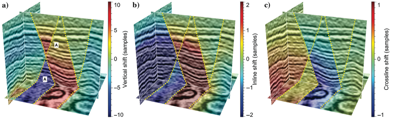
Figure 6. (a) Vertical, (b) inline, and (c) crossline components of unfauling shifts in the unfaulted space are converted from those in the input space shown in Figure 4. The discontinuities on each component of shifts are displaced relative to those in Figure 4.
