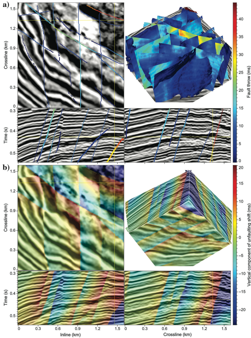
Figure 9. (a) Fault surfaces and slip vectors are first estimated from a 3D seismic image, and they then are used to compute (b) unfauling vector shifts used in image unfauling. Only vertical components of vectors are shown here.
