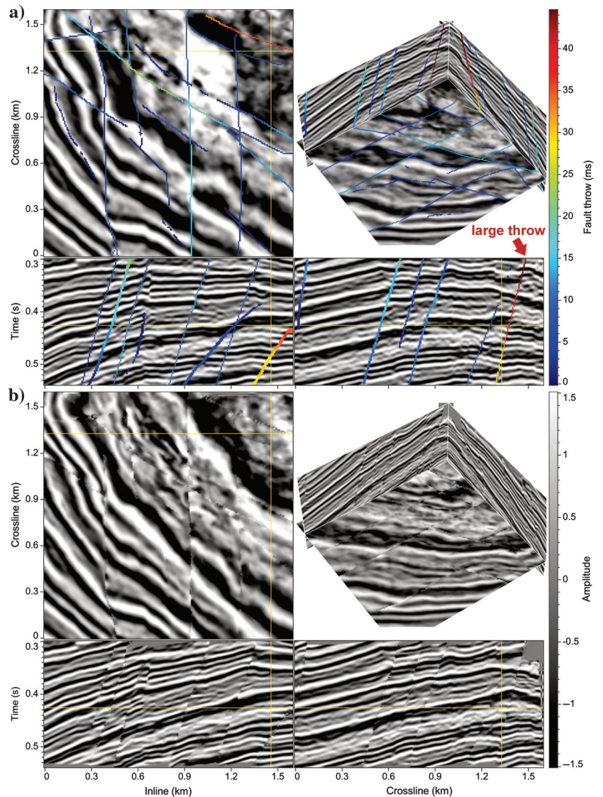
Figure 10. A 3D seismic image (a) before and (b) after unfaulting. In all image slices, seismic reflectors are more continuous after unfaulting. For the large-throw fault highlighted by a red arrow in panel (a), the corresponding fault blocks are significantly moved in panel (b) to align the seismic reflectors on opposite sides of this fault.
