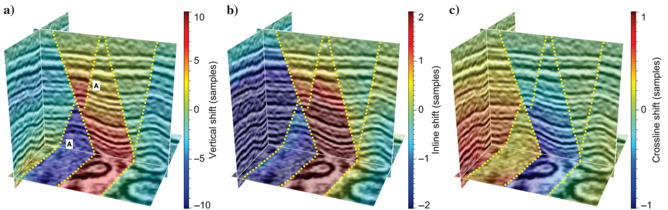
Figure 4. (a) Vertical, (b) inline, and (c) crossline components of unfauling shifts \mathbf{s}(\mathbf{x}) are computed in the input space using method 1. Discontinuities in each component of shifts coincide with fault locations.
